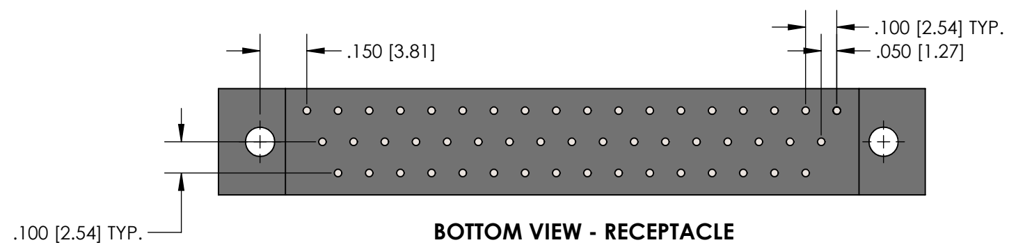
BOTTOM VIEW - RECEPTACLE SIZE 9, 15, 21, 25, 31, AND 37
