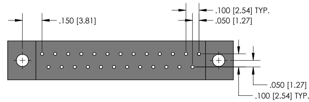
BOTTOM VIEW - RECEPTACLE SIZE 9, 15, 21, 25, 31, AND 37
