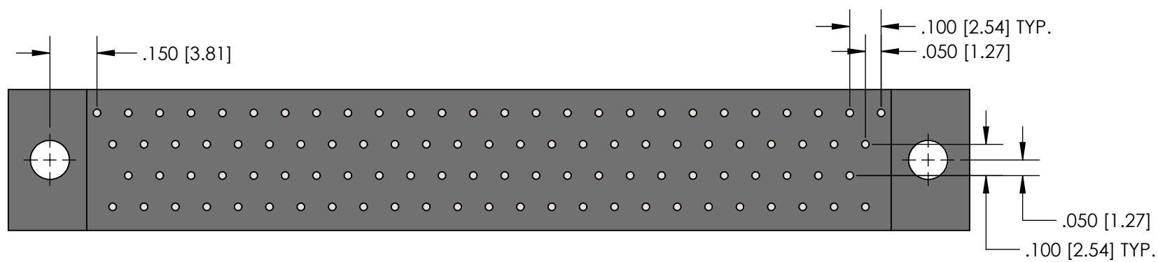
BOTTOM VIEW - RECEPTACLE SIZE 100
