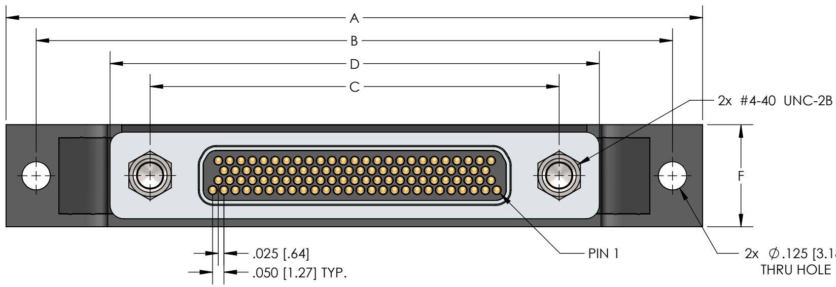
FRONT VIEW - PLUG (PINS)
