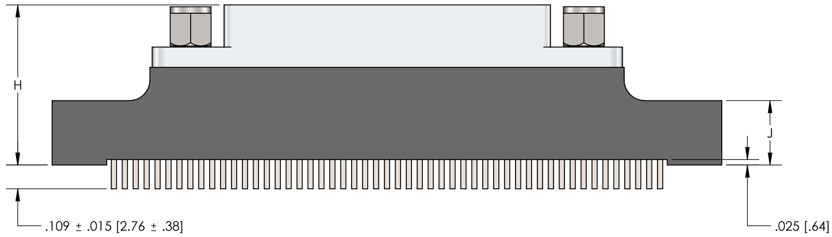
FRONT VIEW - RECEPTACLE (SOCKETS)
